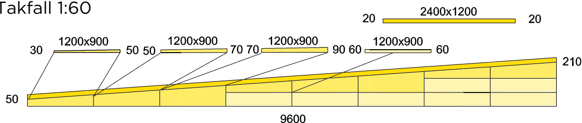
Takfall 1:60
